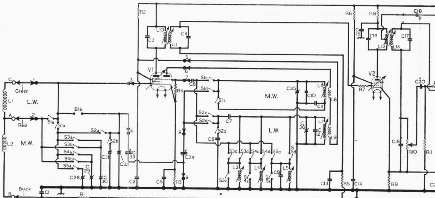
Circuit diagram of the Bush DAC10 A.C./D.C. superhet. No provision is made for the connection of an external aerial. The frame aerial connections are lettered A, B and C , and the connections between the chassis and the tuning unit are numbered 1 to 9 . Note that M.W. is the lower coil in the aerial circuit, and the upper coil in the oscillator.
