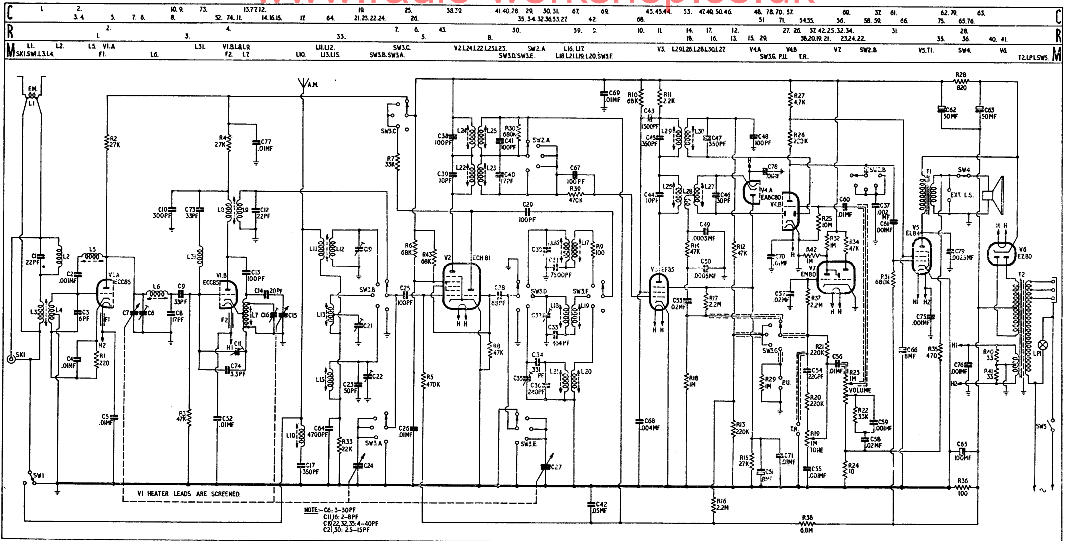
CIRCUIT DIAGRAM
