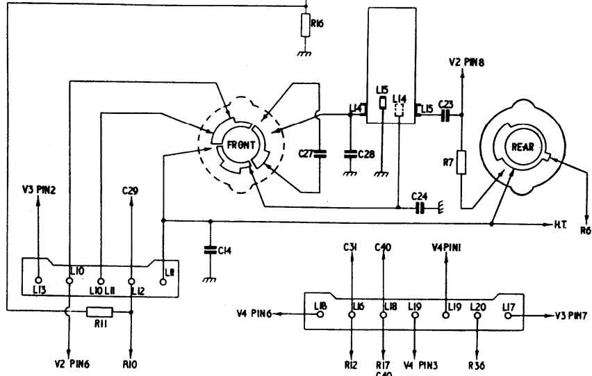
SWITCH & COIL WIRING ALL WAFERS VIEWED FROM REAR WITH CHASSIS INVERTED
