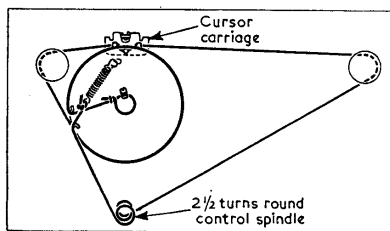
Sketch of the drive cord system.
