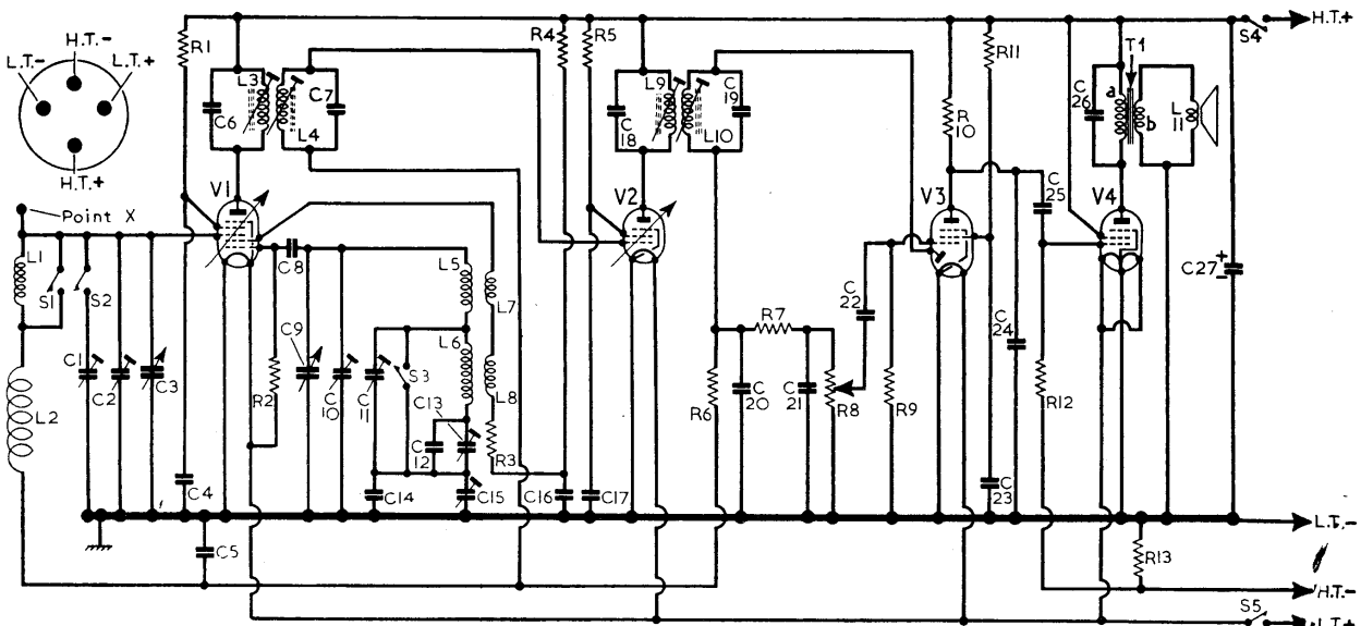
Circuit of Ever Ready "Sky King." Battery plug connections are shown in the top left corner where the plug is viewed from the free ends of its pins.
