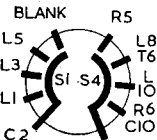
MIDDLE WAFER
