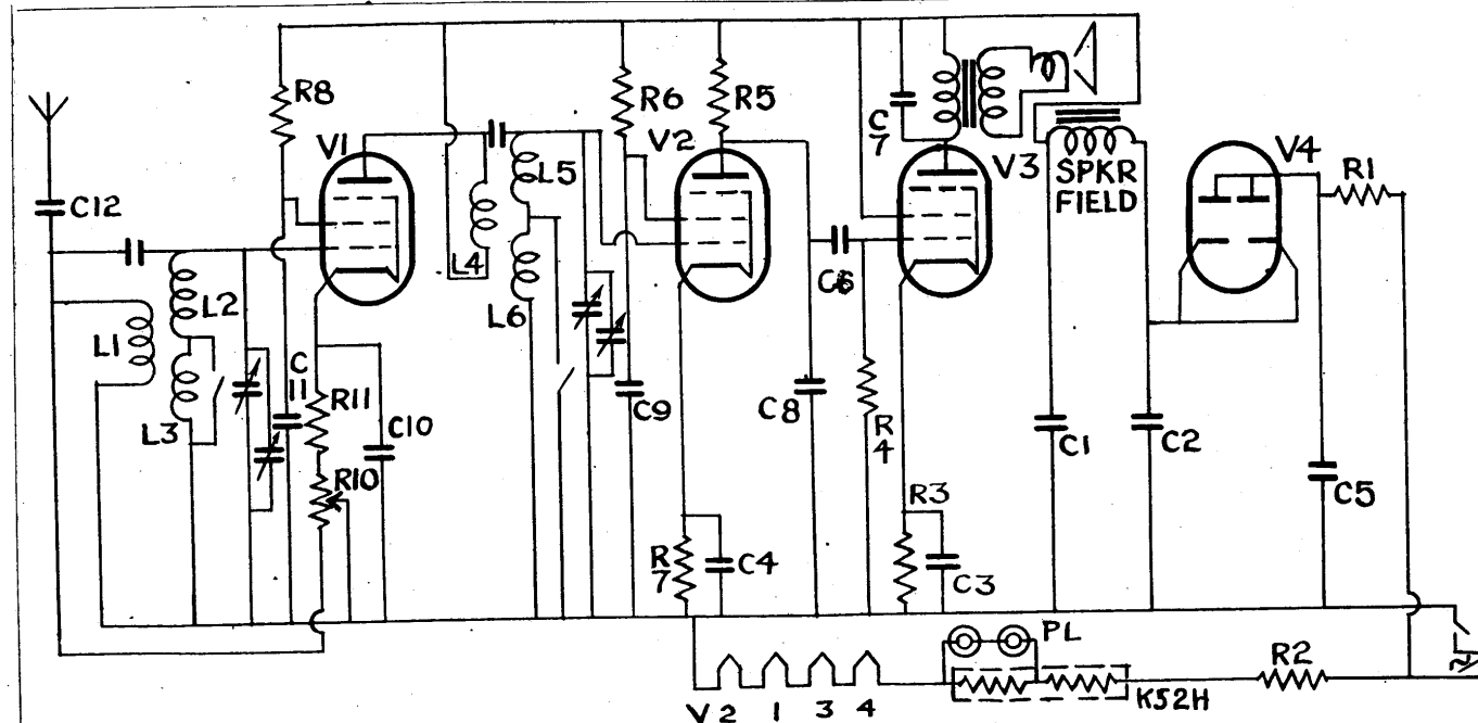
The circuit of the Belmont 550, a midget T.R.F. receiver. Two bands are covered and the detector (V2) is an RF pentode used as an anode-bend rectifier.
