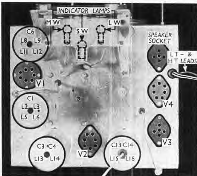
Plan view of the chassis. Note the socket which takes the speaker plug. The trimmers are reached from beneath the chassis, and hence are not indicated on the coil units.
