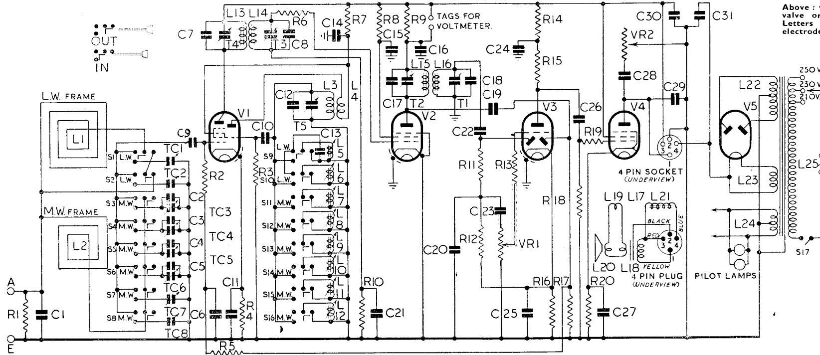
The circuit follows the conventional pattern for a four-valve plus rectifier AC superhet except for the provision of eight push-button circuits in place of the usual switched coils and variable condensers. Frame aerials are fitted but an external collector can be connected.
