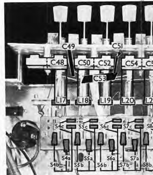
The tuning unit as seen from the underside of the cabinet. The scale lamp and indicator button tuning are all clear
