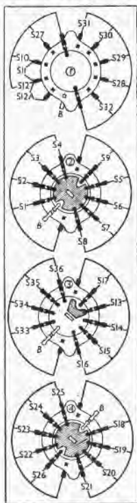
Switch diagrams, looking at the underside of the chassis in the directions of the arrows in the under-chassis view. The switches formed by the metal plates on the rotors of units 2 to 4 are omitted for clarity.
