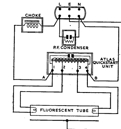
Fig. 12.—Quickstart single 80W circuit
