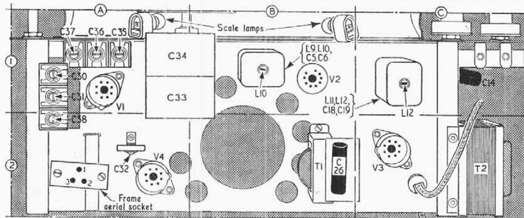
Plan view of chassis, showing the vertically mounted trimmer C32 which in the early version models takes the place where we show C31, this trimmer being replaced by a fixed capacitor. The frame aerial socket is a 2-pin type in the early versions.
