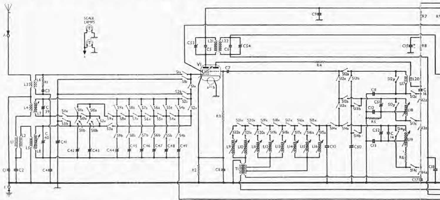
Circuit diagram of the Marconiphone 874 and H.M.V. 1102. In the press-button section, condenser trimmers are used for the aerial coils for the oscillator circuit. V1 is the double-diode AFC discriminator valve, which has two separate cathodes. T1 is the AFC control transformer; its pick-up socket is split.
