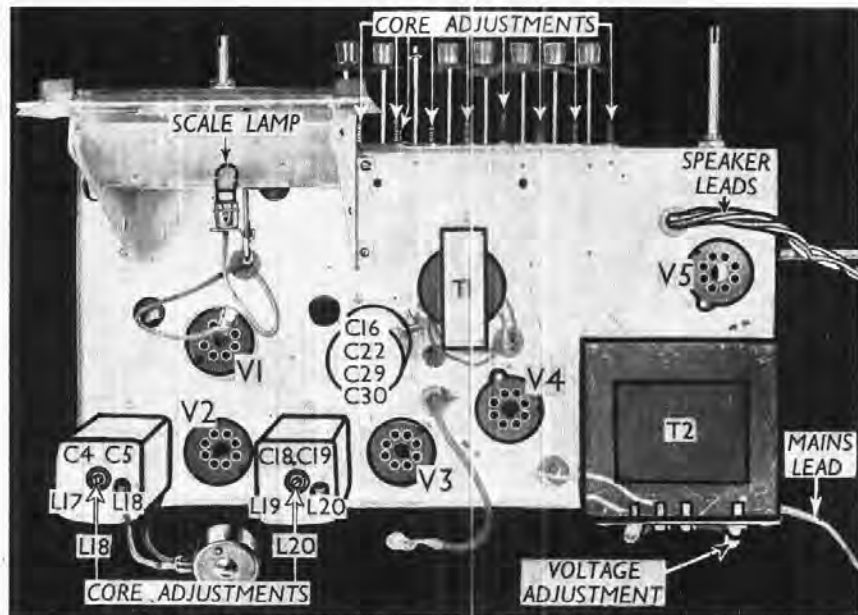
Plan view of the chassis. The core adjustments of the IF transformer secondary coils are indicated; the primary adjustments are beneath the chassis.
