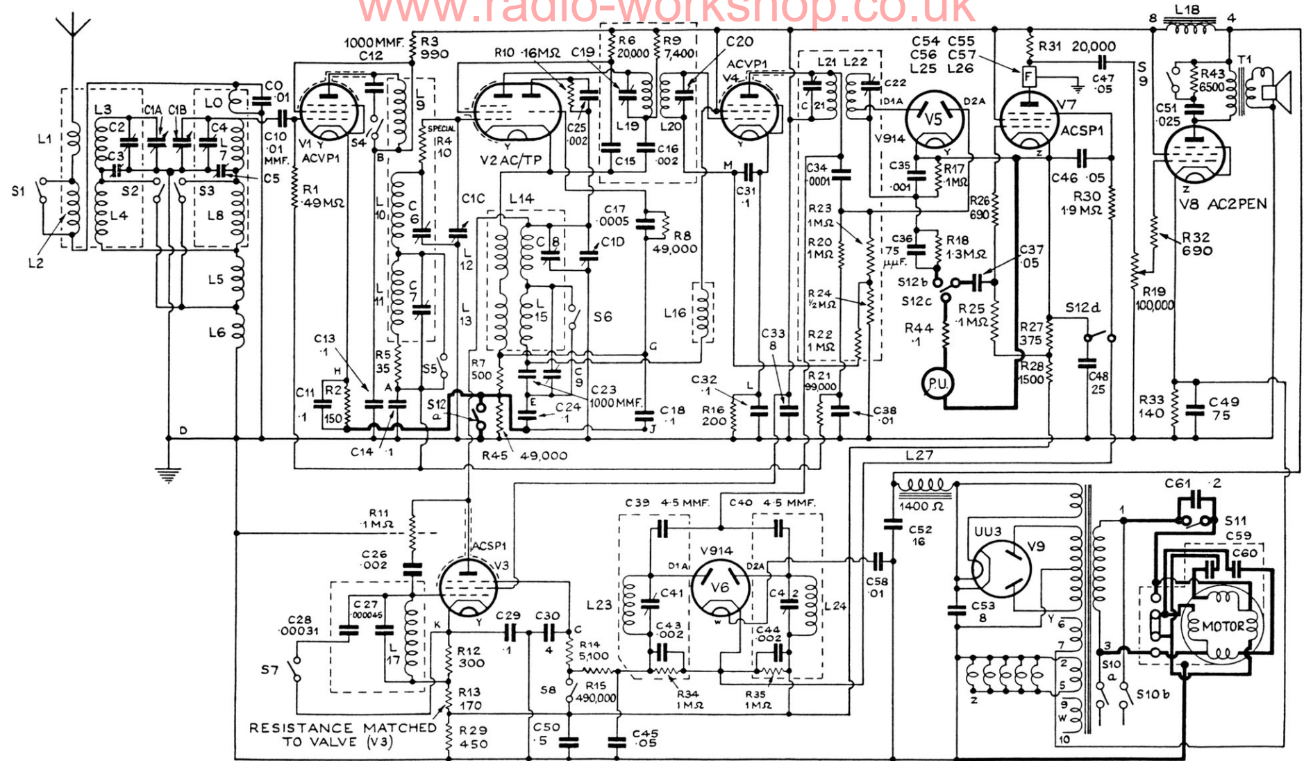
A28RG CIRCUIT DIAGRAM
