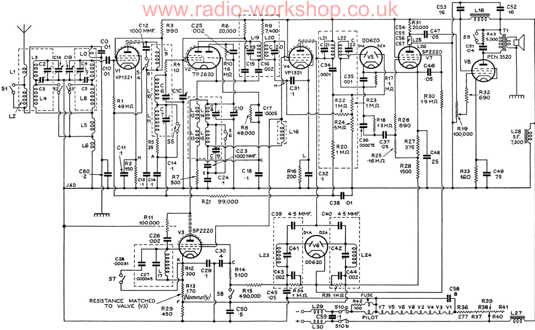
D28C CIRCUIT DIAGRAM
