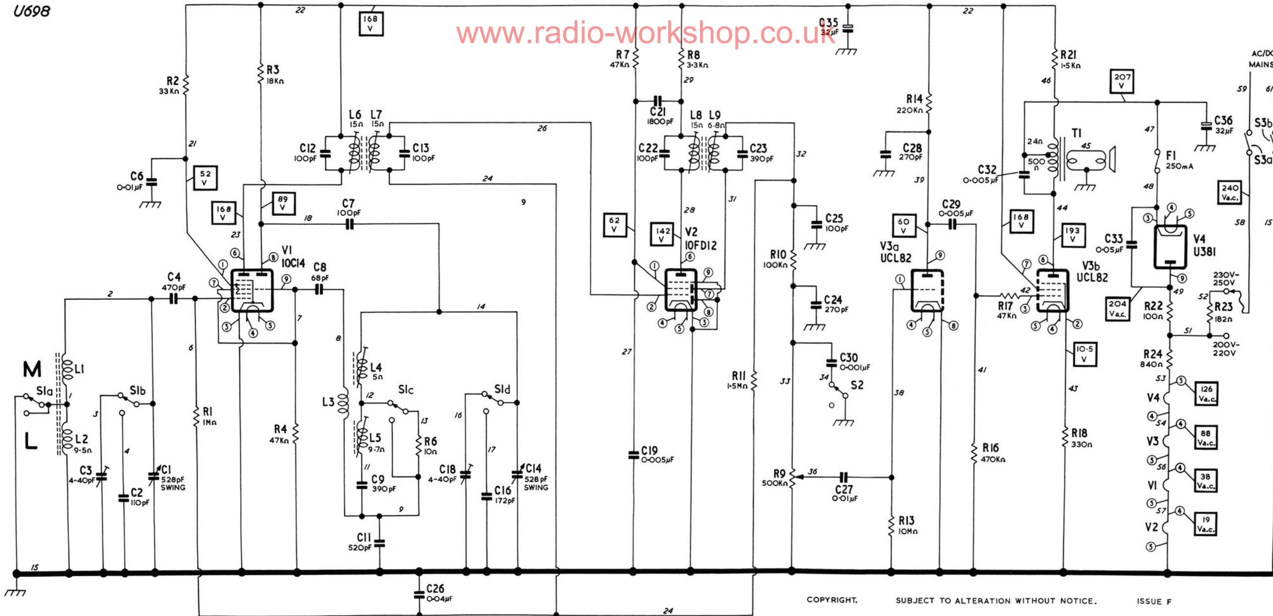
Fig. 2. The circuit diagram.
