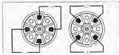
Diagrams showing the base connections of the two M.W. and L.W. coil units.
