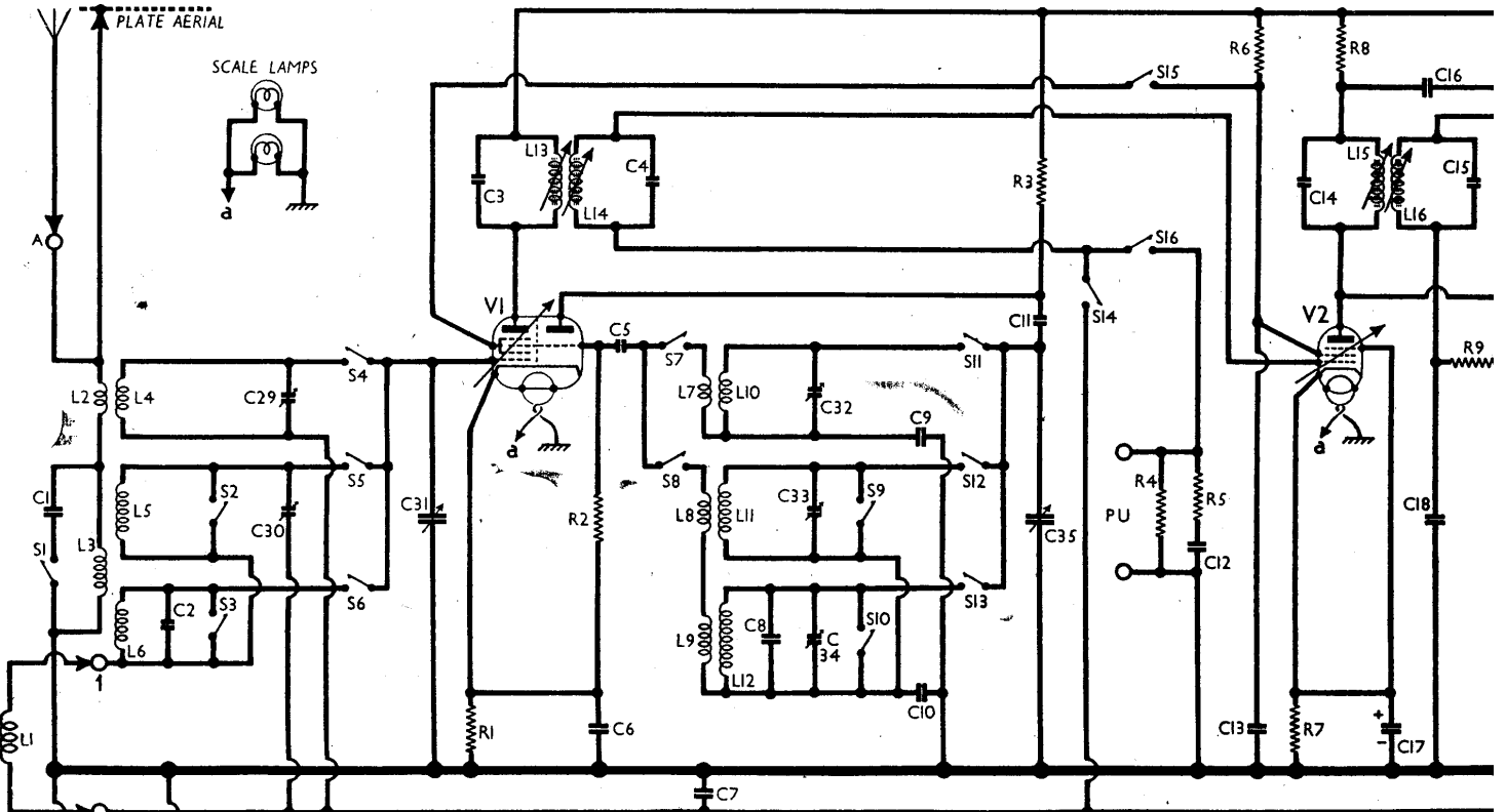
Circuit diagram of the Pye 18A 3-band superhet. L1 is the frame aerial winding. S1 opens automatically when is inserted. The G18K autoradiogram circuit is only slightly different, but several component values are changed iron-cored choke. In the export versions, the mains transformer primary is as shown inset just to the left of V4. plug (the range selector) joins points A and B to points C and D respectively for 100 v mains, or simply B to C for (voltage selector) plug selects one of the tappings E, F or G.
