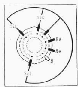
Diagram of the tone control switch unit, as seen from the rear of an inverted chassis. Below is the associated table.
