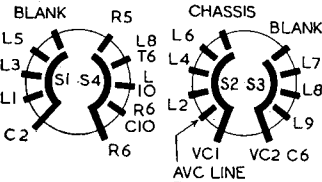
MIDDLE WAFER
