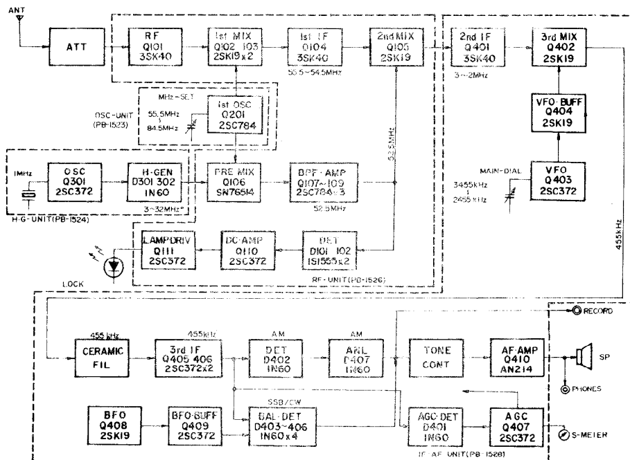
Fig 3 BLOCK DIAGRAM
