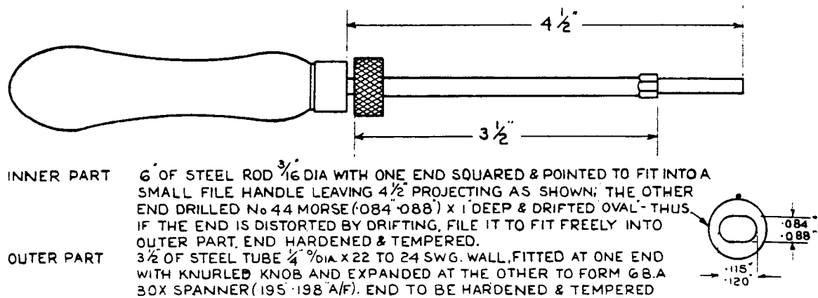
Fig. 12. Ganging Tool.
