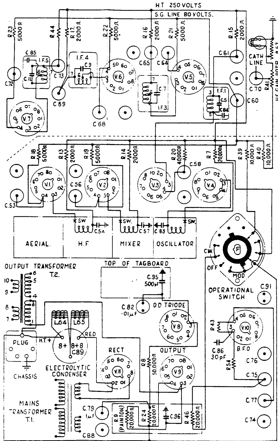
H.T. Circuits.
