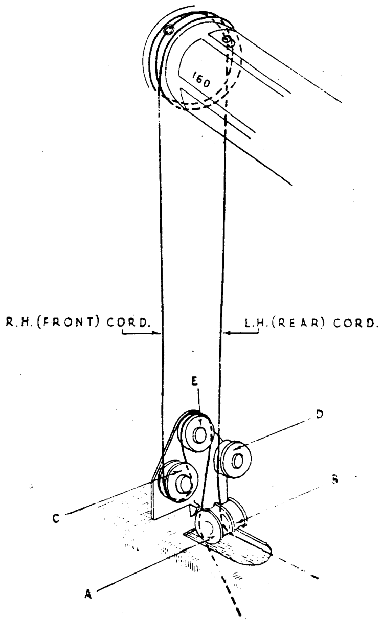
Fig. 11. Band-change Cord.
