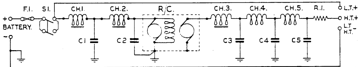
Diagram of Connections, Rotary Converter and Battery.
