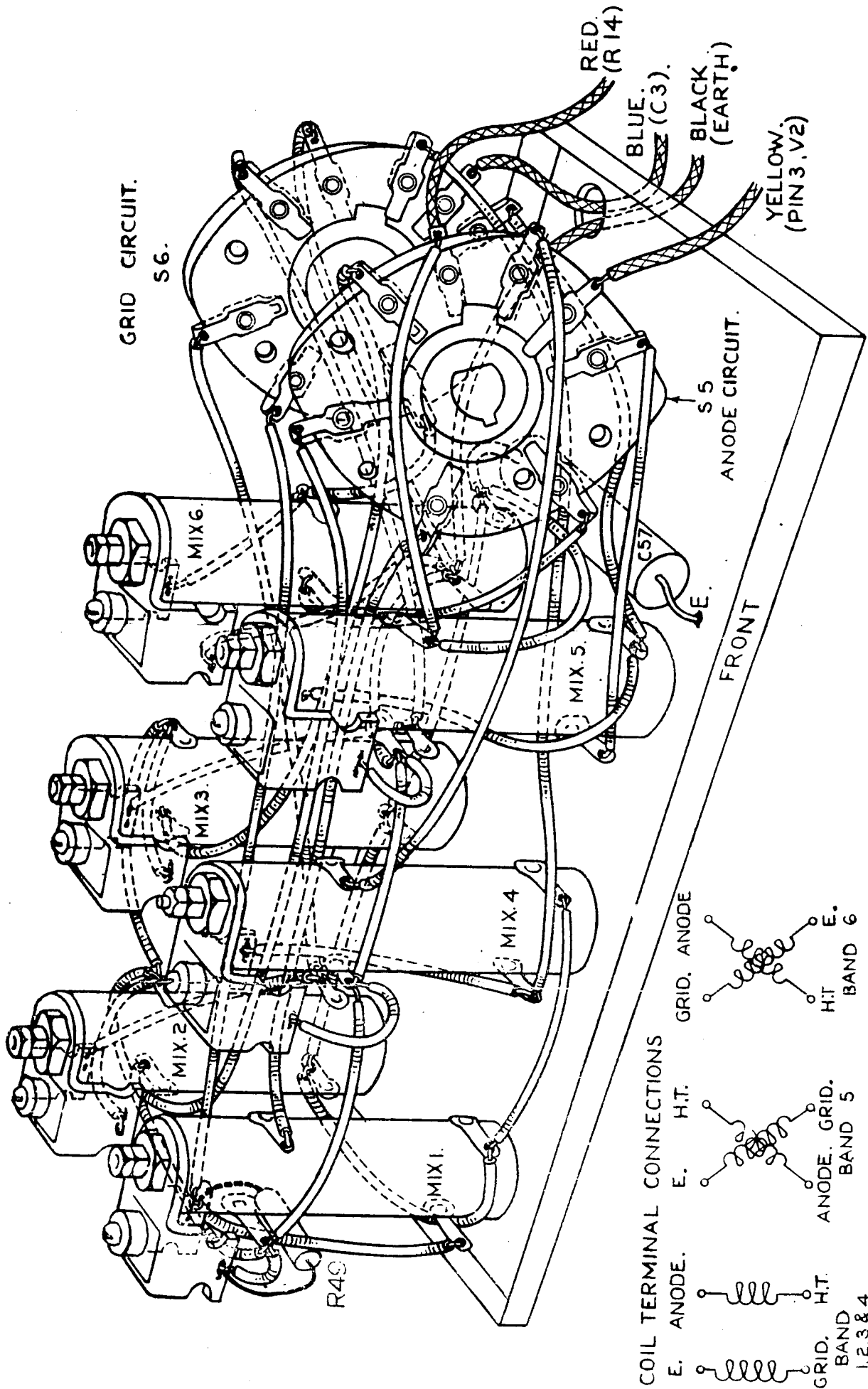
Fig. 24. COIL ASSEMBLY. MIXER SECTION.
