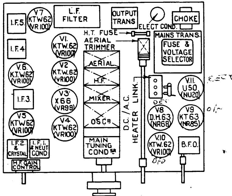
Fig. 3. Plan showing Valve Positions.
