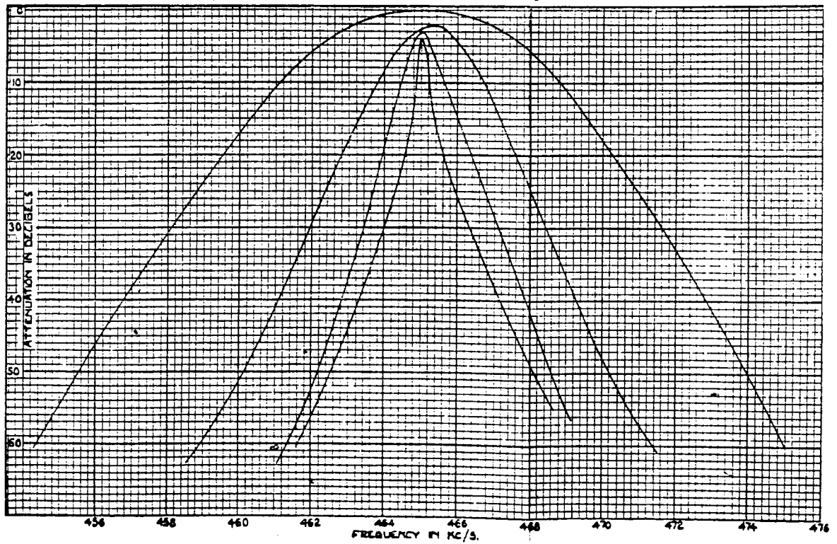
Fig. 5. I.F. Response Curves.
