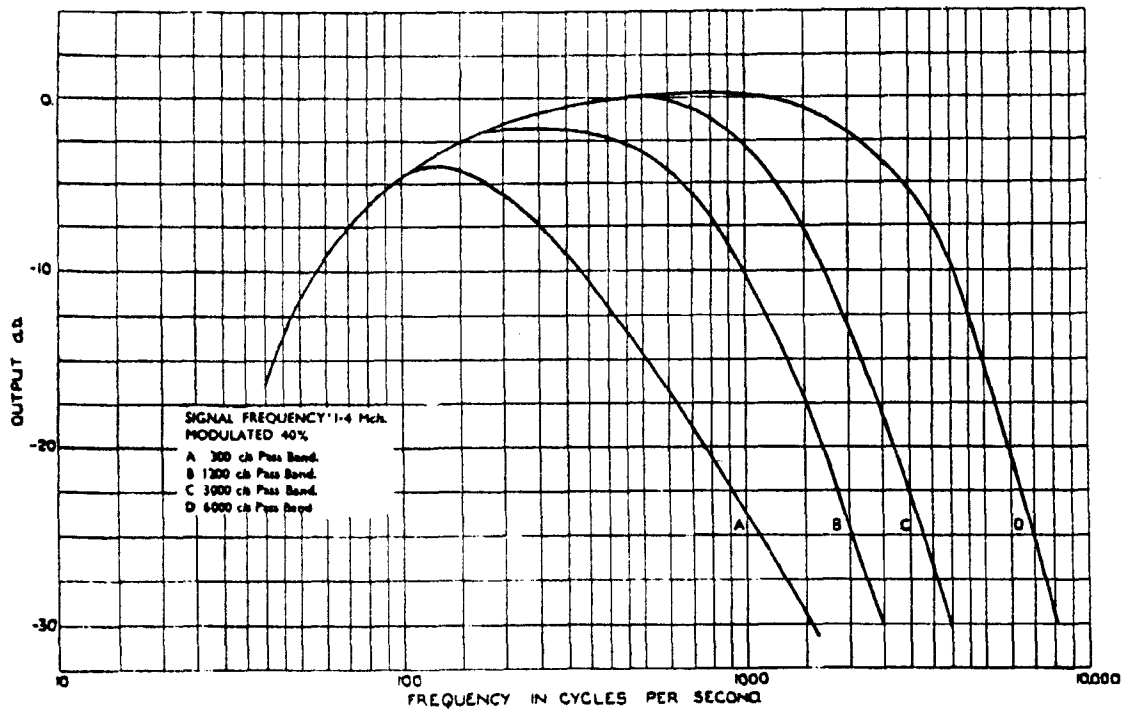
Fig. 8. Overall Fidelity Response Curves.
