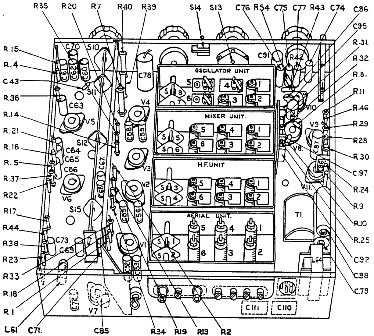
Fig. 21. UNDERNEATH OF CHASSIS.
