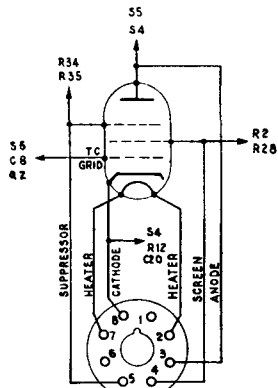
V.1 KTW. 61 (FOM CR.300/2) OR ARTH. 2 (FOM CR.300/1) VARIABLE-MU. HF. PENTODE.
